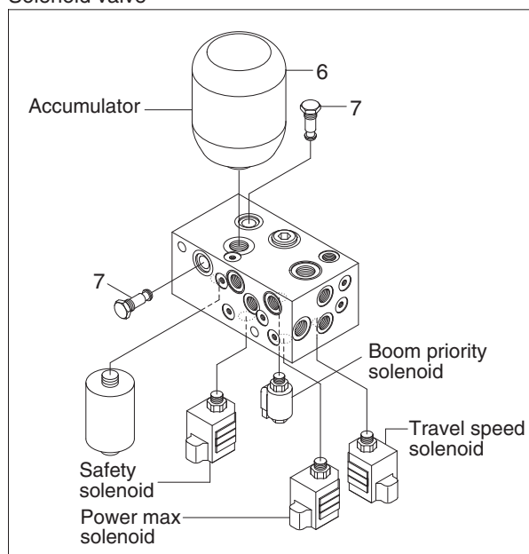
Solenoid valve
