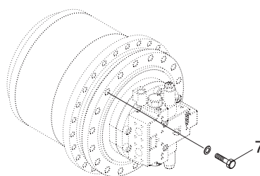
Travel motor
